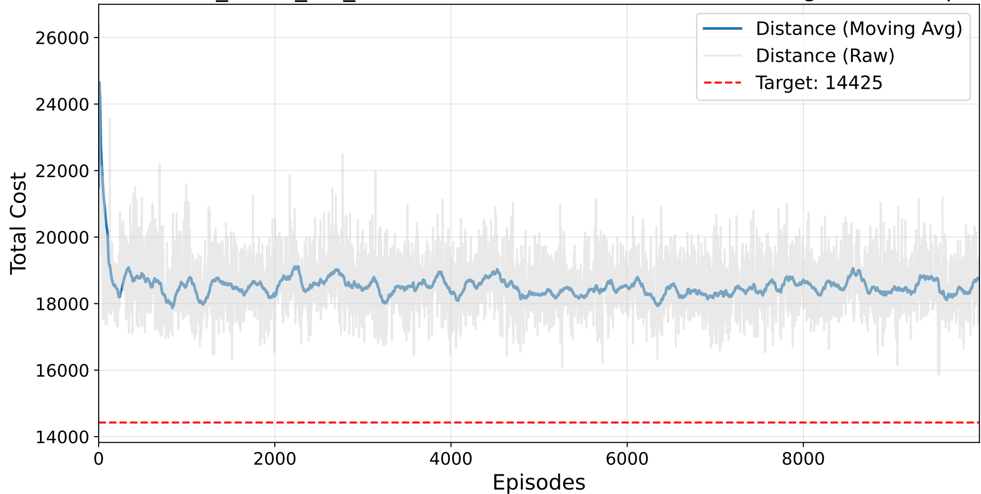
Final NO_MASK_NO_BAYESIAN Masked AutoRL-SOP Training - ft53.4.sop
